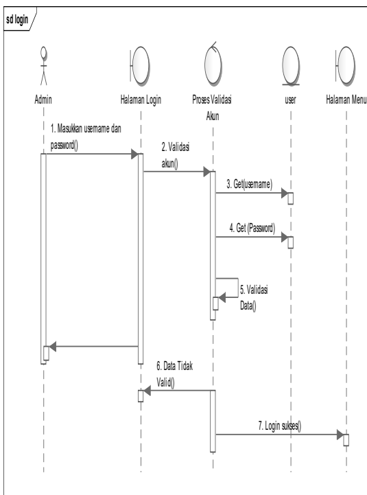
Gambar 4. Sequence Diagram Login
