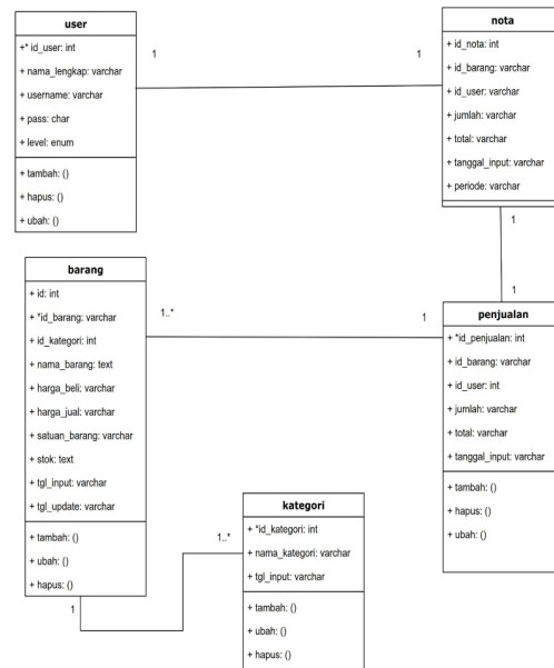
Gambar 6. Class Diagram
