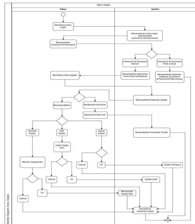
Gambar 7. Activity Diagram Menu Gejala
